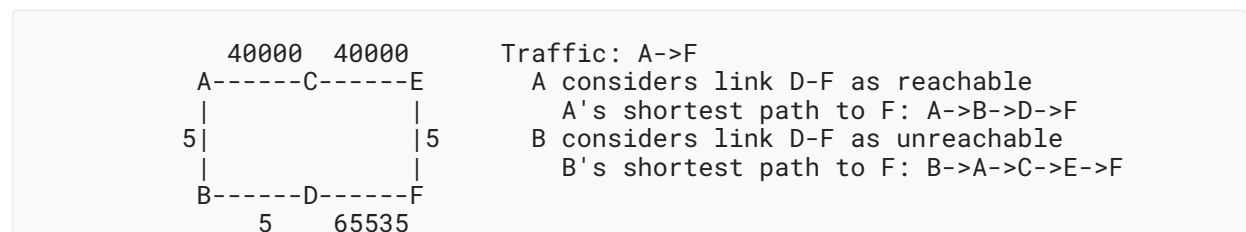
Figure 5: Inconsistent LSLinkInfinity Interpretation Causing Loops
